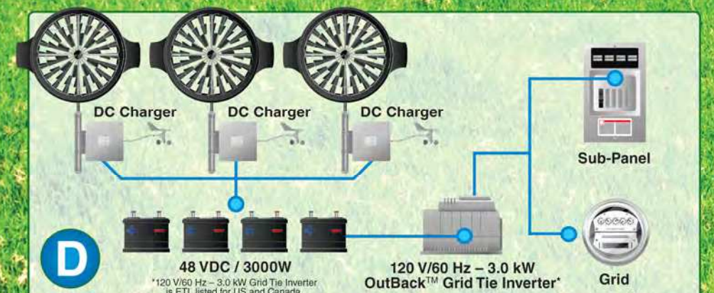
Grid Tie utility connection – up to 3 turbines per OutBack™ Inverter, operational during power failure
