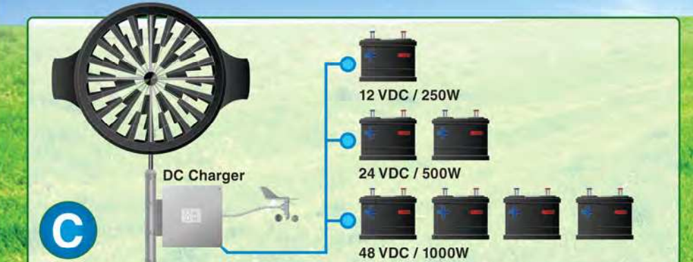
Direct DC 12/24/48 V battery charging
