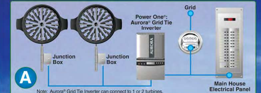
Grid Tie easy connection to utility – up to 2 turbines per Aurora® Inverter, no batteries required
